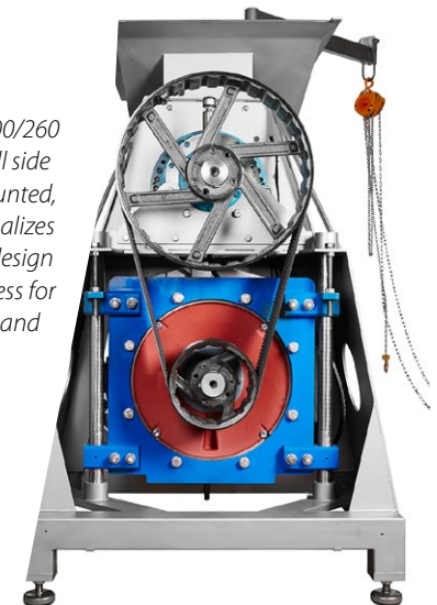
SuperGrind 400/260 shown with all side panels dismantled, side view. Designed for easy access at maintenance and inspection. The automatic greasing system for main bearing and front bearing is also shown.
