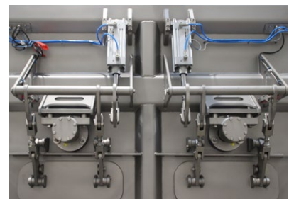
scansteel foodtech® Twin Shaft Mixer discharge gate system.
