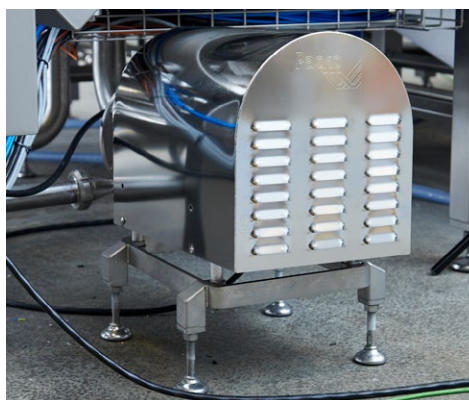
Pumps are positioned/mounted on their own frame for easy access at inspection/maintenance, etc. In addition, the pump of the scanGravy mixing unit can be equipped with its own knife system for eliminating lumps in “challenging to produce” gravies.
